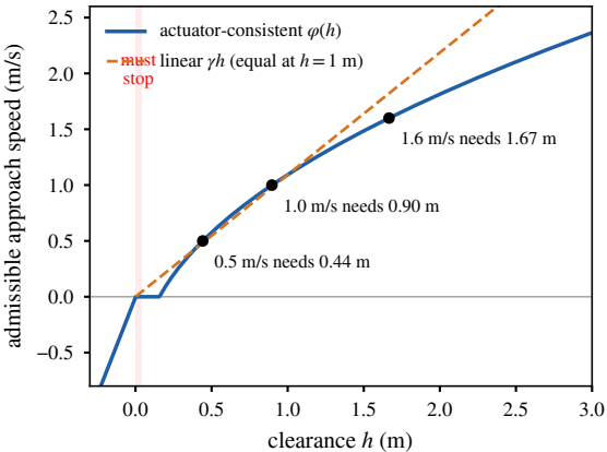
(a) class- \mathcal{K} function, static rows
